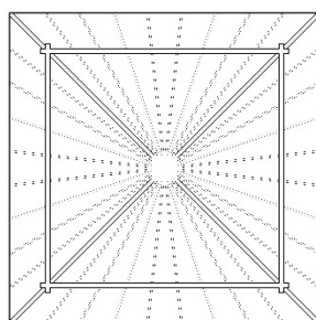
23 Blueprint Umbrella House © DEHLI GROLIMUND All Umbrella House plans are redrawn from the original working drawings and verified against the originals on behalf of the Kazuo Shinohara Estate.
