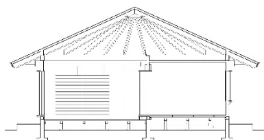
22 Blueprint Umbrella House © DEHLI GROLIMUND All Umbrella House plans are redrawn from the original working drawings and verified against the originals on behalf of the Kazuo Shinohara Estate.
