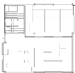
25 Blueprint Umbrella House © DEHLI GROLIMUND All Umbrella House plans are redrawn from the original working drawings and verified against the originals on behalf of the Kazuo Shinohara Estate.
